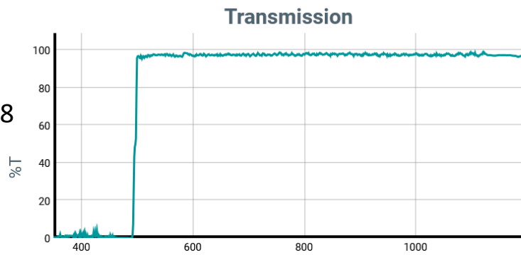
Filter F49-605
